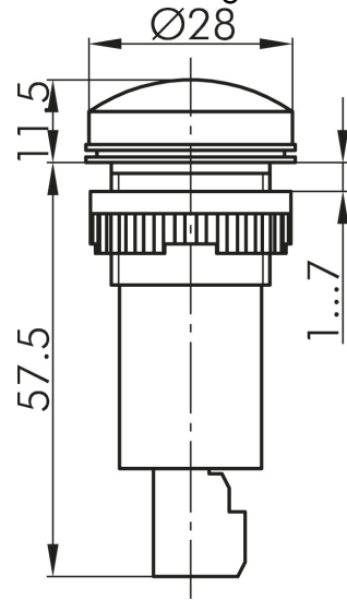
Dimensional drawing:
