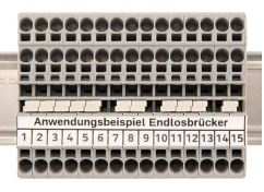
Continuous jumpers (2002 Series) readily connect an endless number of terminal blocks to each other via single jumper slot. Use the second jumper slot for additional commoning or testing.
