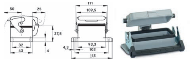
EPIC® H-B 16 AG Housing design H-B. The industry standard.
