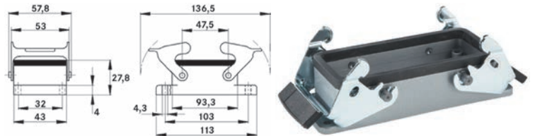
EPIC® H-B 16 AG Housing design H-B. The industry standard.
