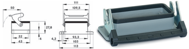
EPIC® H-B 16 AD-LB Housing design H-B. The industry standard.
