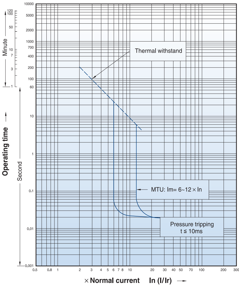
Magnetic trip units(MTU)
