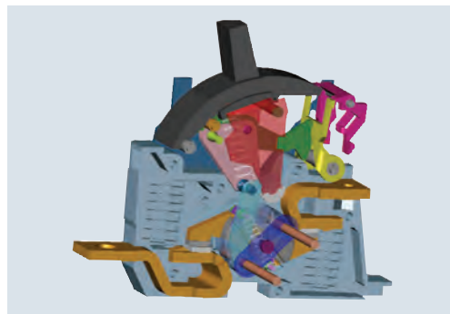
Fig. 3 "ON" position
