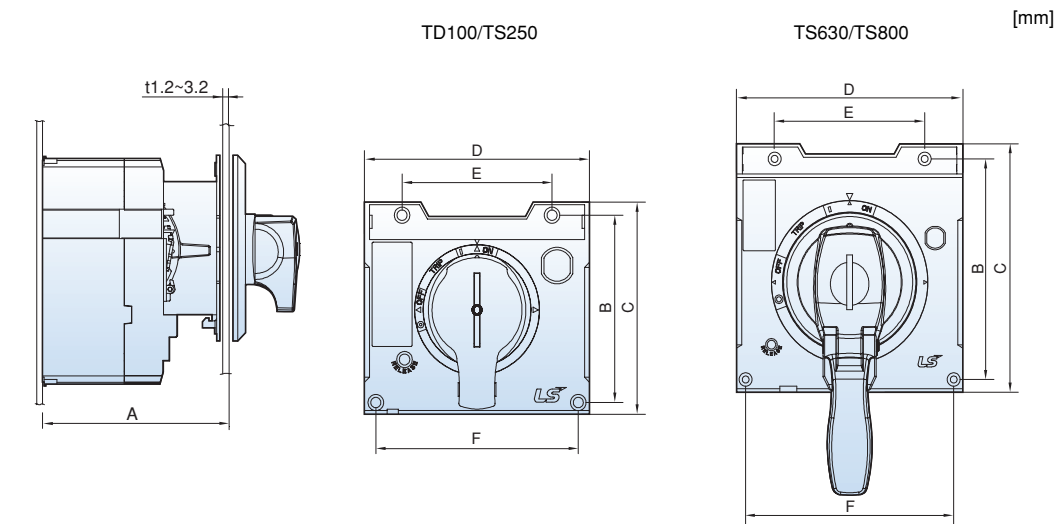
Dimension table for D-handles
