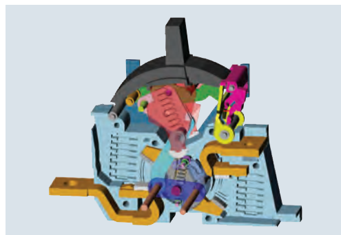
Fig. 5 "TRIP" position
